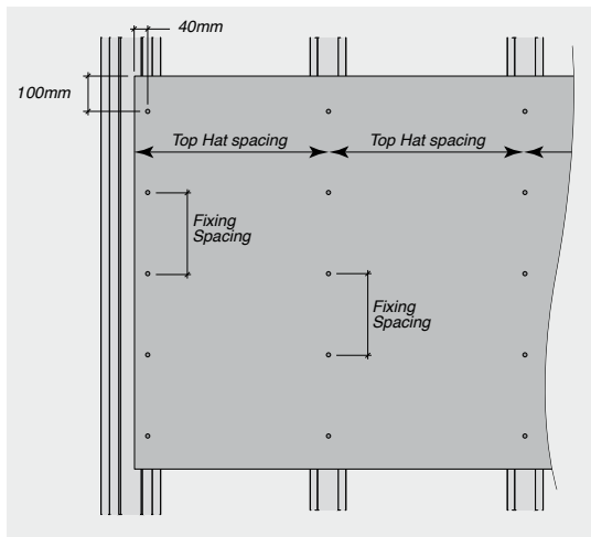
FIGURE 6.08 Horizontal Sheet Fixing
