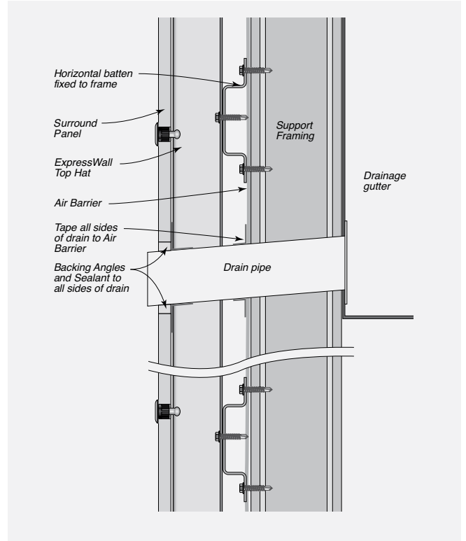
FIGURE 8.22 Typical Drain
