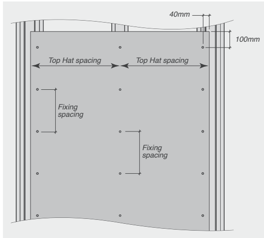
FIGURE 6.07 Vertical Sheet Fixing
